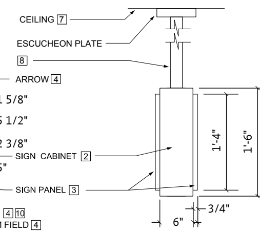
2 END ELEVATION NOT TO SCALE
