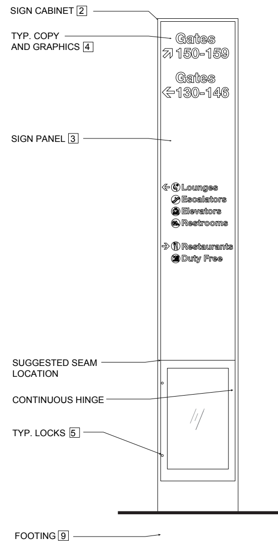
4 ELEVATION (SIDE B) NOT TO SCALE
