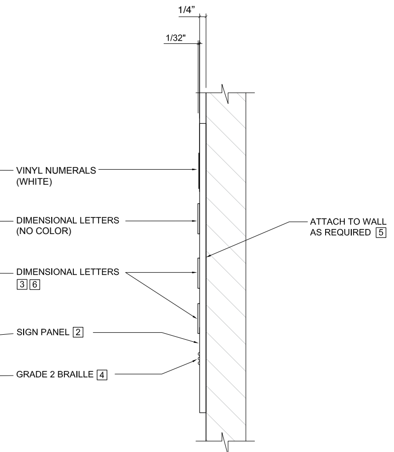
2 Side Elevation NOT TO SCALE
